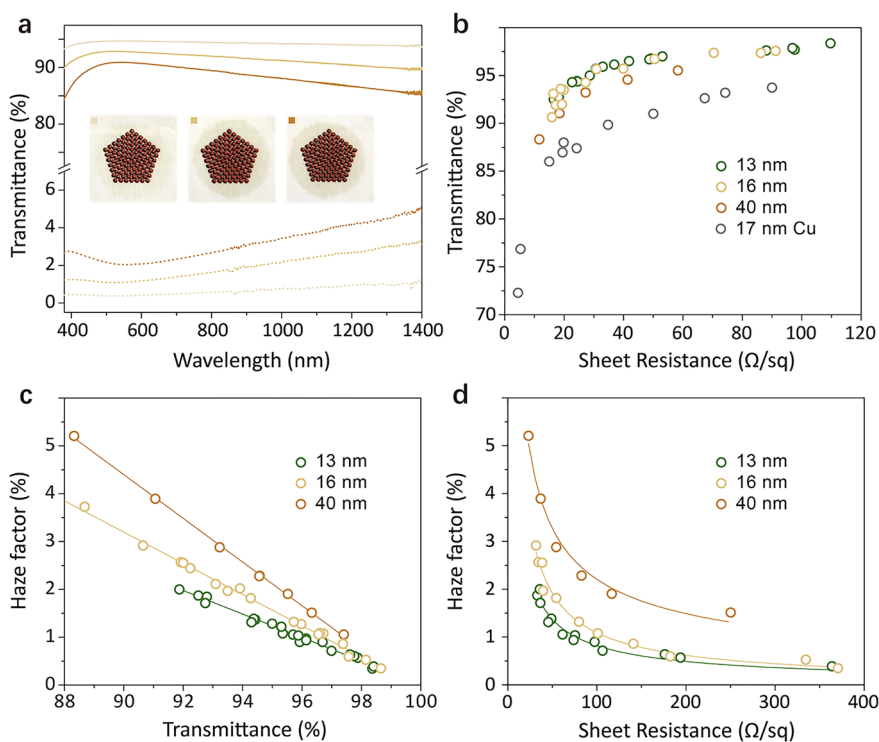
Figure 4. Optoelectronic performance of transparent conductive films. (a) transmittance (solid curve) and scattering (dashed curve) spectra of transparent conductors with different loadings of 13 nm silver nanowires. Inset shows the optical pictures of films in the corresponding cases. Plots of transmittance versus sheet resistance (b), haze factor versus transmittance (c), and haze factor versus sheet resistance (d) of electrodes made with silver nanowires with different mean diameters.
